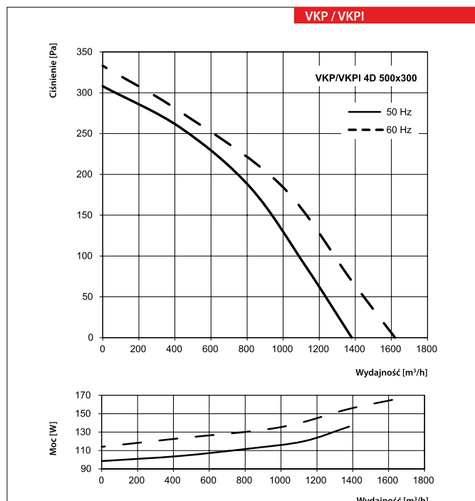
VKP 4D 500x300
